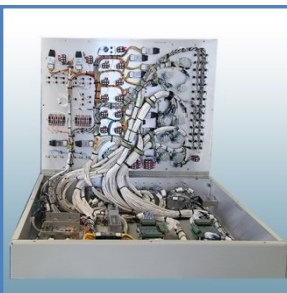
Switching Sub-Assembly
